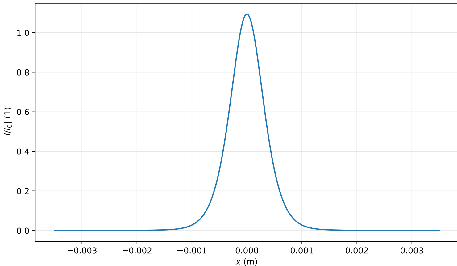
Intensity profile I(x, y = 0, z = 3.025m)/I_0 , P_{in}=0.8P_{cr} , artificial time
